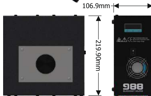
Model 988 Application Part of an airport fever detection system.
